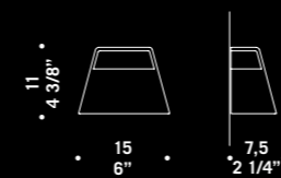
DIAPHANÈS A15 1xMAX 3,5W G9 LED LED light bulb
